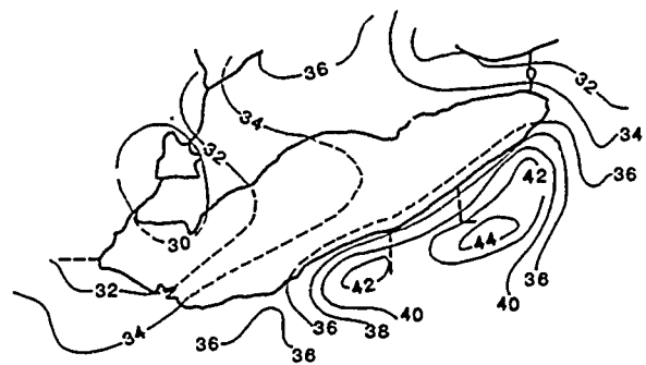
Figure 4.9. Mean annual precipitation (inches). (Redrawn from Phillips and McCulloch, Chart 21)
