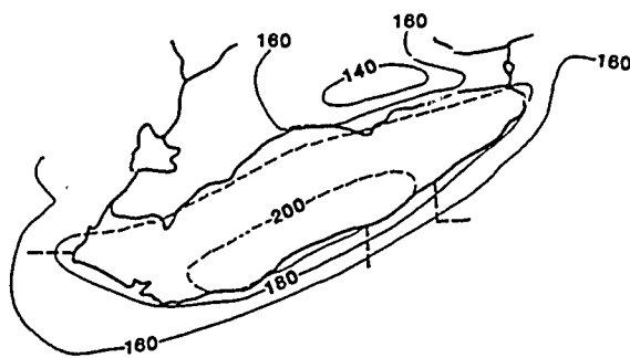
Figure 4.8. Mean annual frost-free period (days). (Redrawn from Phillips and McCulloch, Chart 19)
