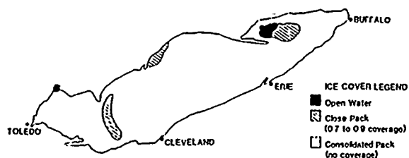
Figure 4.5. Normal winter maximum ice cover, Feb. 20-28. (Redrawn from Donald R. Ronly, Great Lakes Ice Atlas . NOAA Technical Memorandum LSCR 1, Sept., 1971, Plate 26.)
